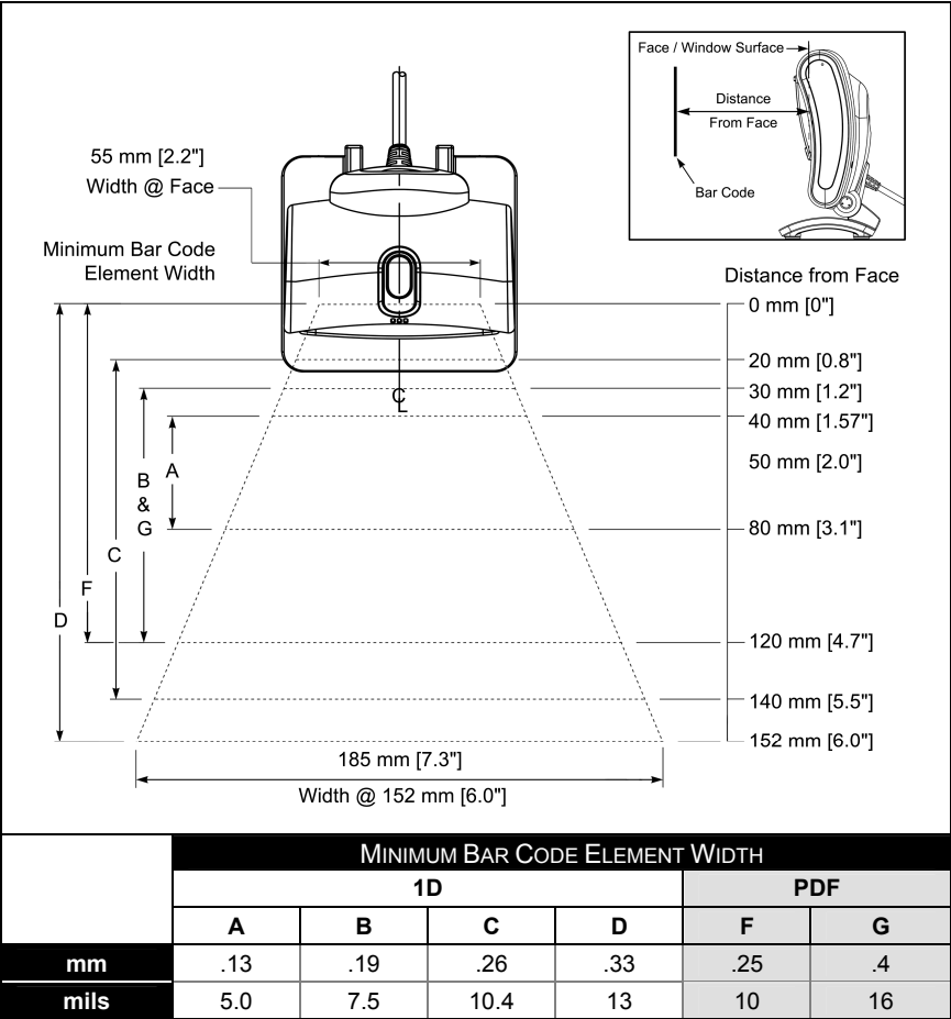
Figure 20. Depth of Field by Minimum Bar Code Element Width
